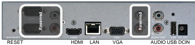
Back Panel Connectors
